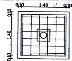
PLAN OF FOOTING
